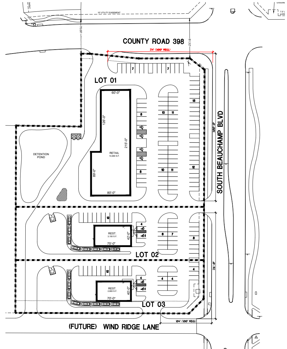
EXAMPLE SITE PLAN #2
